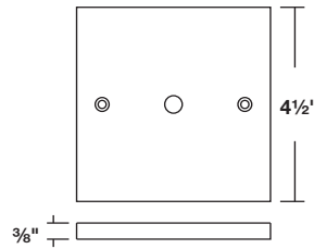
P-1171-01 SQUARE BACKPLATE
